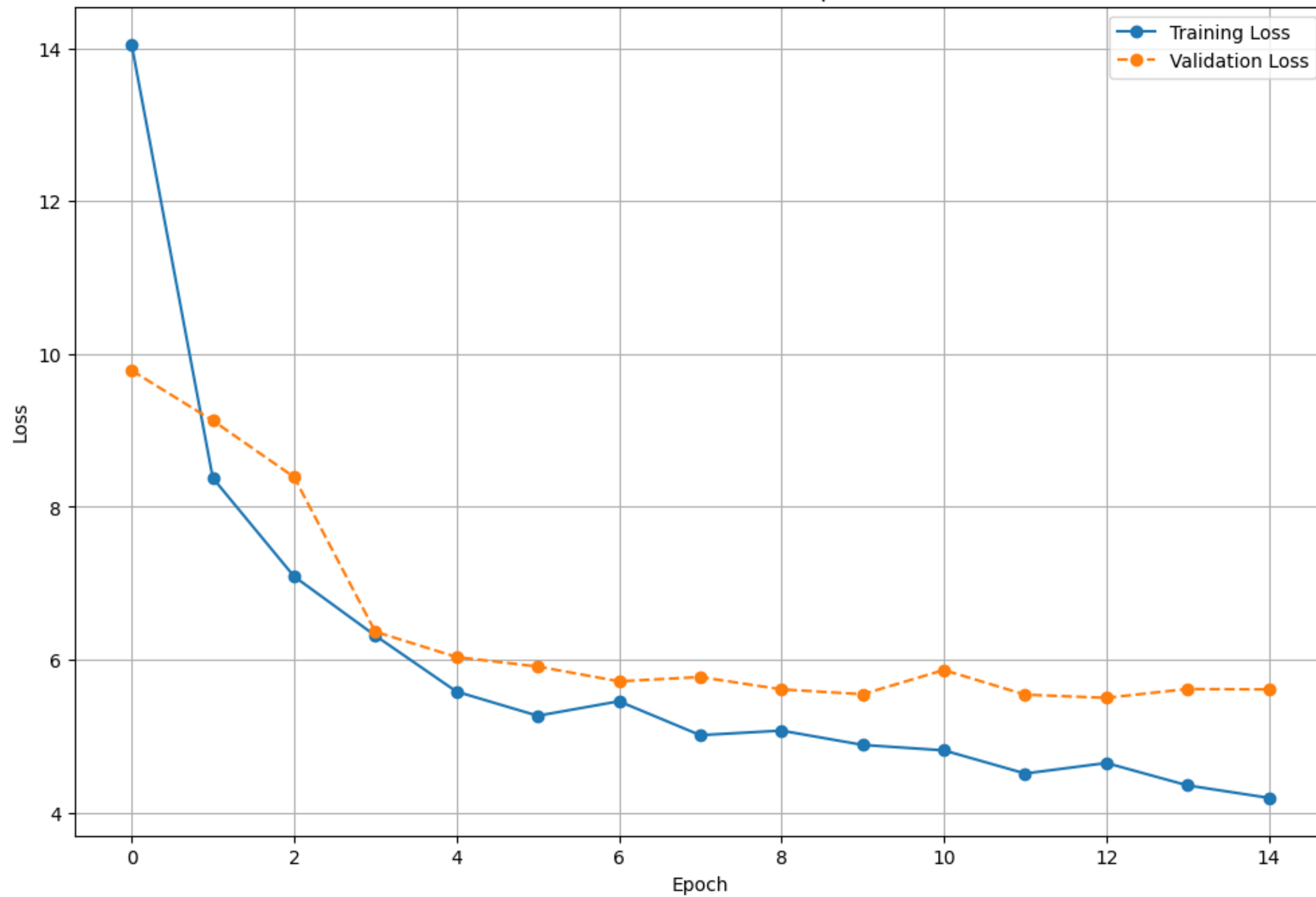
Train/Validation Loss over Epochs
